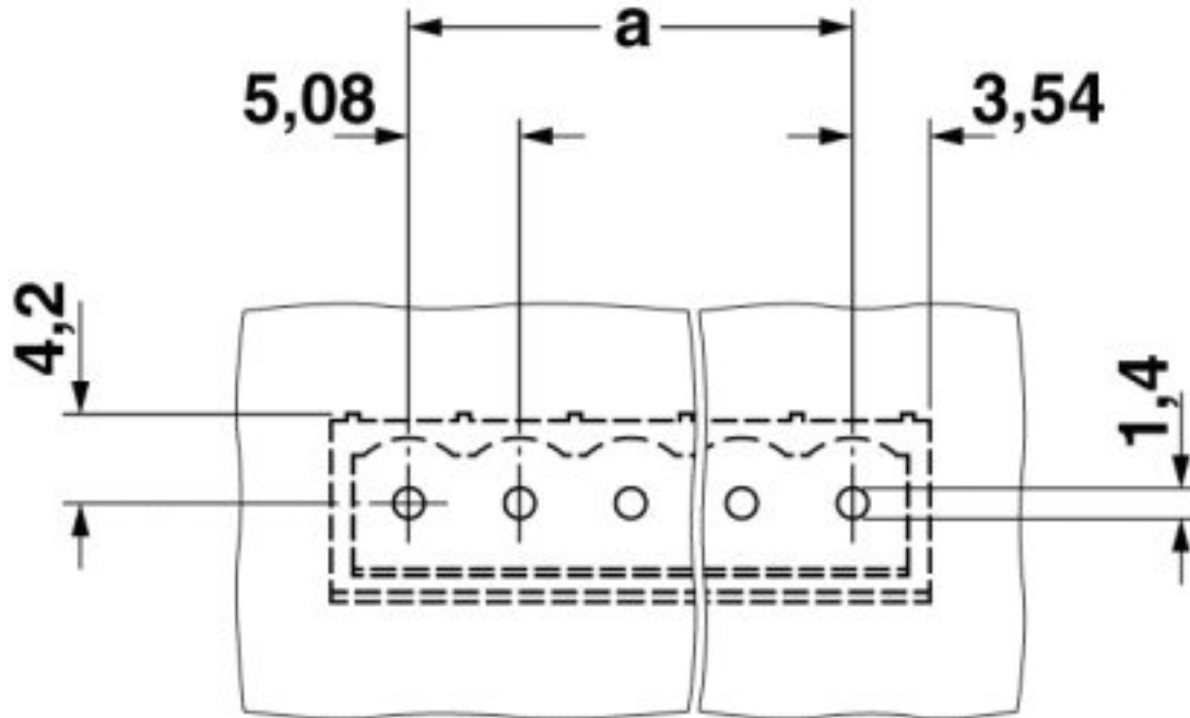
Drilling diagram
